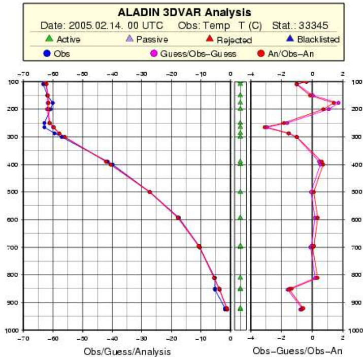
figure 13.: profiles of different quantities (obs, guess, analysis, obs-guess, obs-analysis) for a given analysis at the location of a radiosonde observation. The status of the observations is also indicated.
