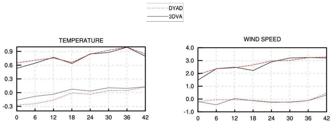
figure 2.: RMSE and BIAS of the temperature and wind forecasts on 500hPa
