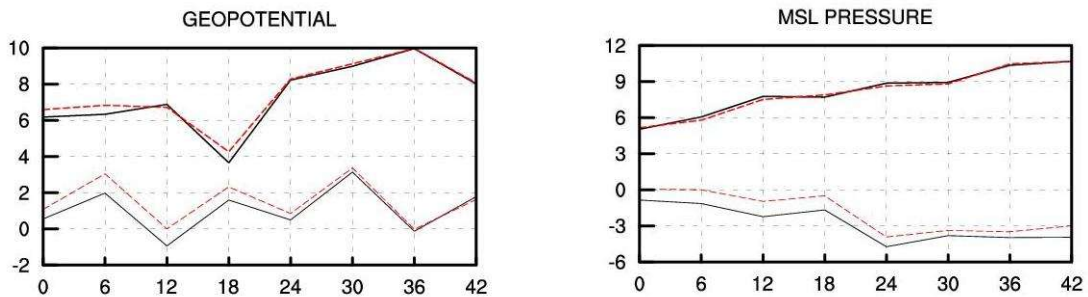
figure 3.: RMSE and BIAS of geopotential on 700hPa (left) and mean sea level pressure (right)
