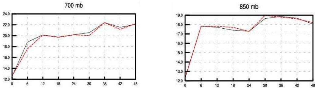
figure 8.: Impact of AMSU-B data on relative humidity (RMSE scores). HUN2: operative model, TEST2: AMSU-B parallel suite
