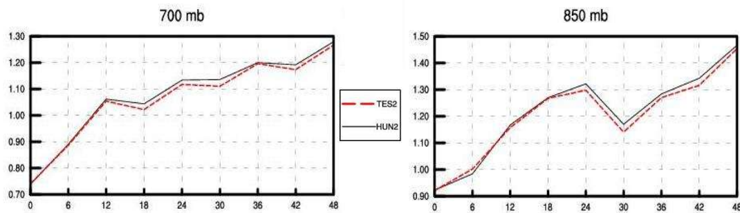
figure 7.: Impact of AMSU-B data on low level temperature (RMSE scores). HUN2: operative model, TEST2: AMSU-B parallel suite
