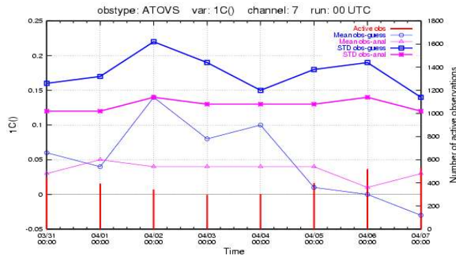
figure 11: time evolution of the different properties (mean and standard deviation of obs – guess and obs - analysis, number of active observations) of the ATOVS/AMSU-A data (channel 7)
