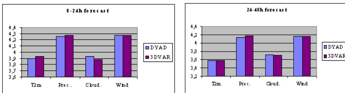
figure 5.: subjective scores of the dynamical adaptation (DYAD) and the assimilation system (3DVAR) for the first (left) and the second (right) day of the forecast (period: 01.07.2004 – 31.12.2004)
