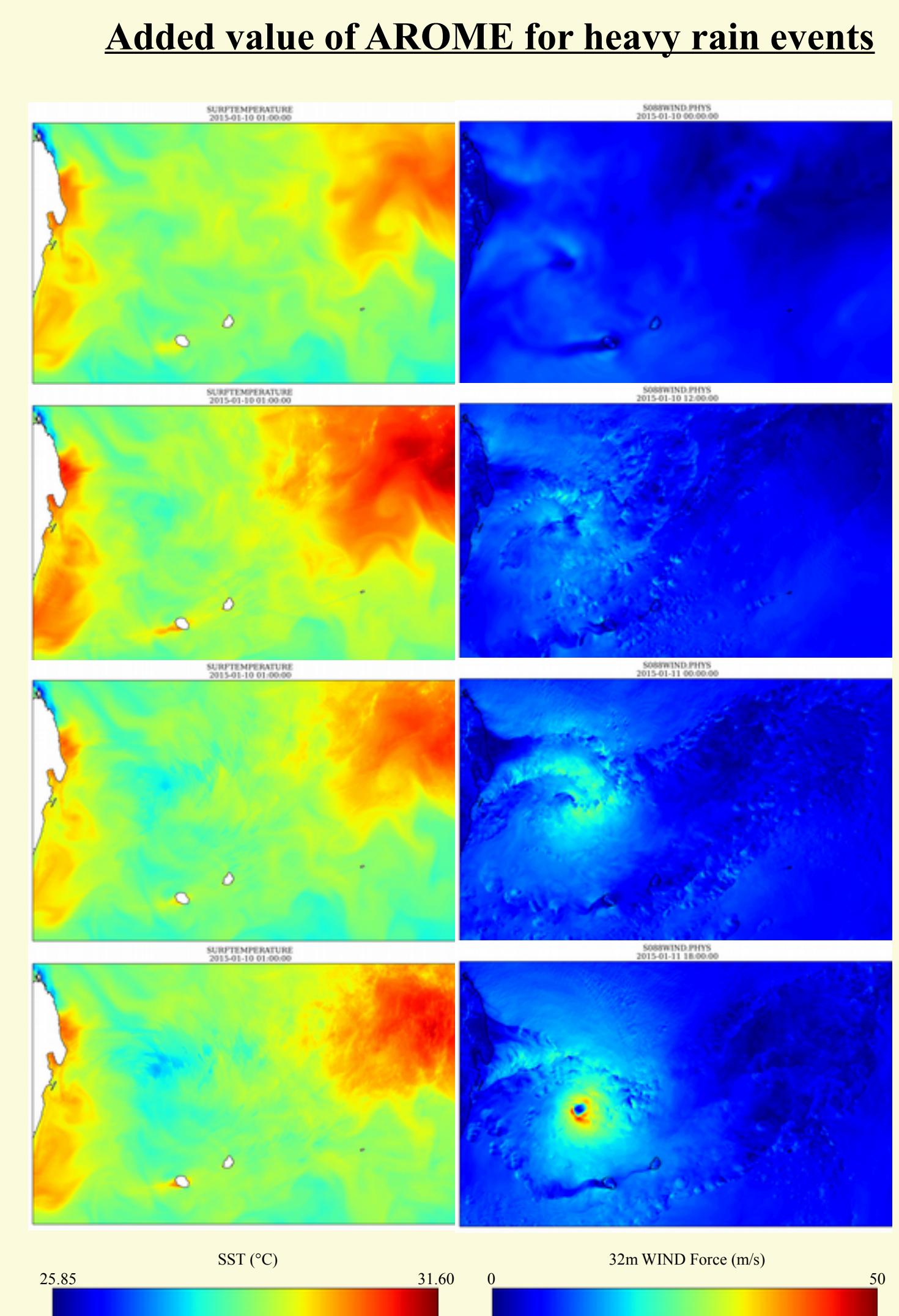
Figure 13 : AROME over Indian Ocean, Tropical Cyclone Bejisa, AROME +42h forecast based on 2013/12/31 0h run
