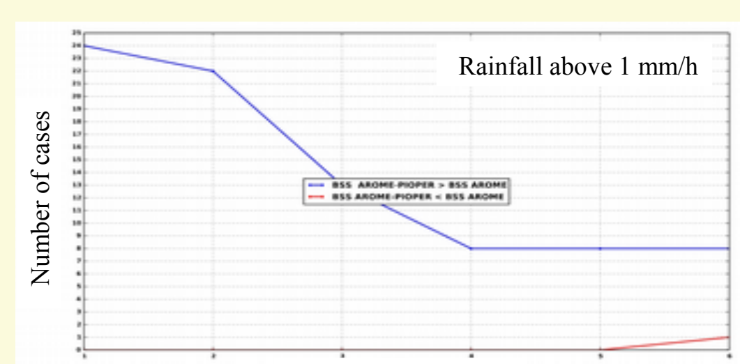
Figure9: From the 30th August 2015 to the 7th December 2015, the classical AROME-France with longer cut-off (from 15 minutes to 3 hours) and later time delivery (from 1 to 4 hours after initial time) has been compared to AROME-PI.
